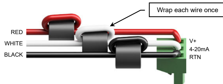
FIGURE 4.3.3 POWER WIRES W/ FERRITE BEADS INSTALLED
